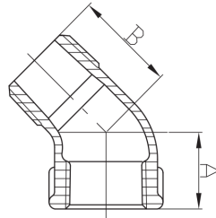
45° Street Elbow
